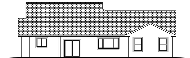
Back Elevation
